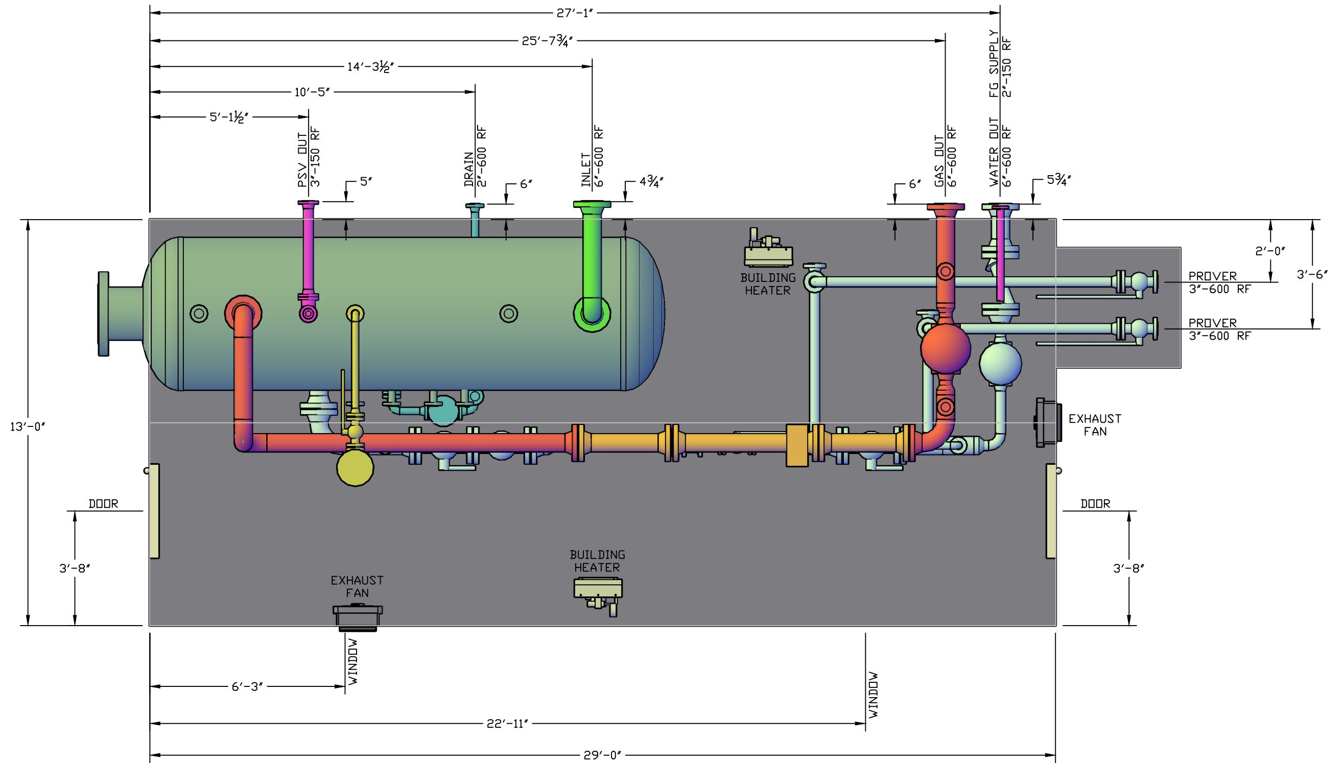
TOP VIEW
