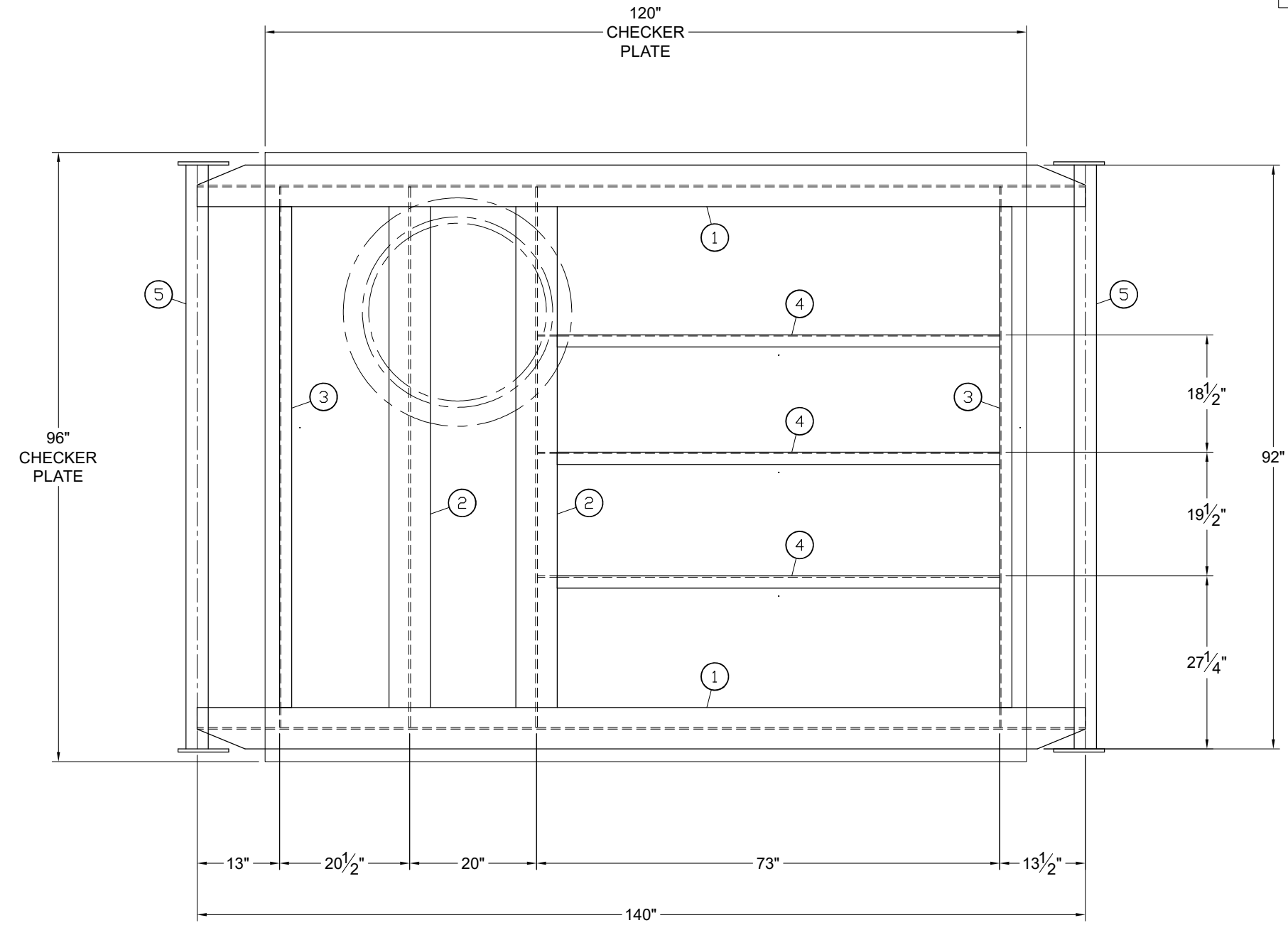
PLAN VIEW
